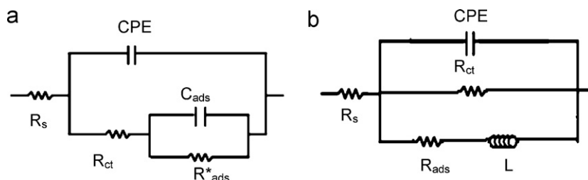
Fig. 12. Electrical equivalent circuit diagram used for modeling electrocatalyst/solution interface in 1.00 M CH 3 OH + 1.00 M KOH for Ni-promoted Cd/C (a) and Ni/C (b) catalysts, respectively. R_p = R_{ct} + R_{ads} ( R^*_{ads} ), R_s : solution resistance; R_{ct} : charge transfer resistance; R^*_{ads} : surface adsorption resistance; R_{ads} : resistance of adsorbed specimen (electroactive constituents, methanol); CPE: double layer capacitance; C_{ads} : related to the adsorption process; L : inductance.
