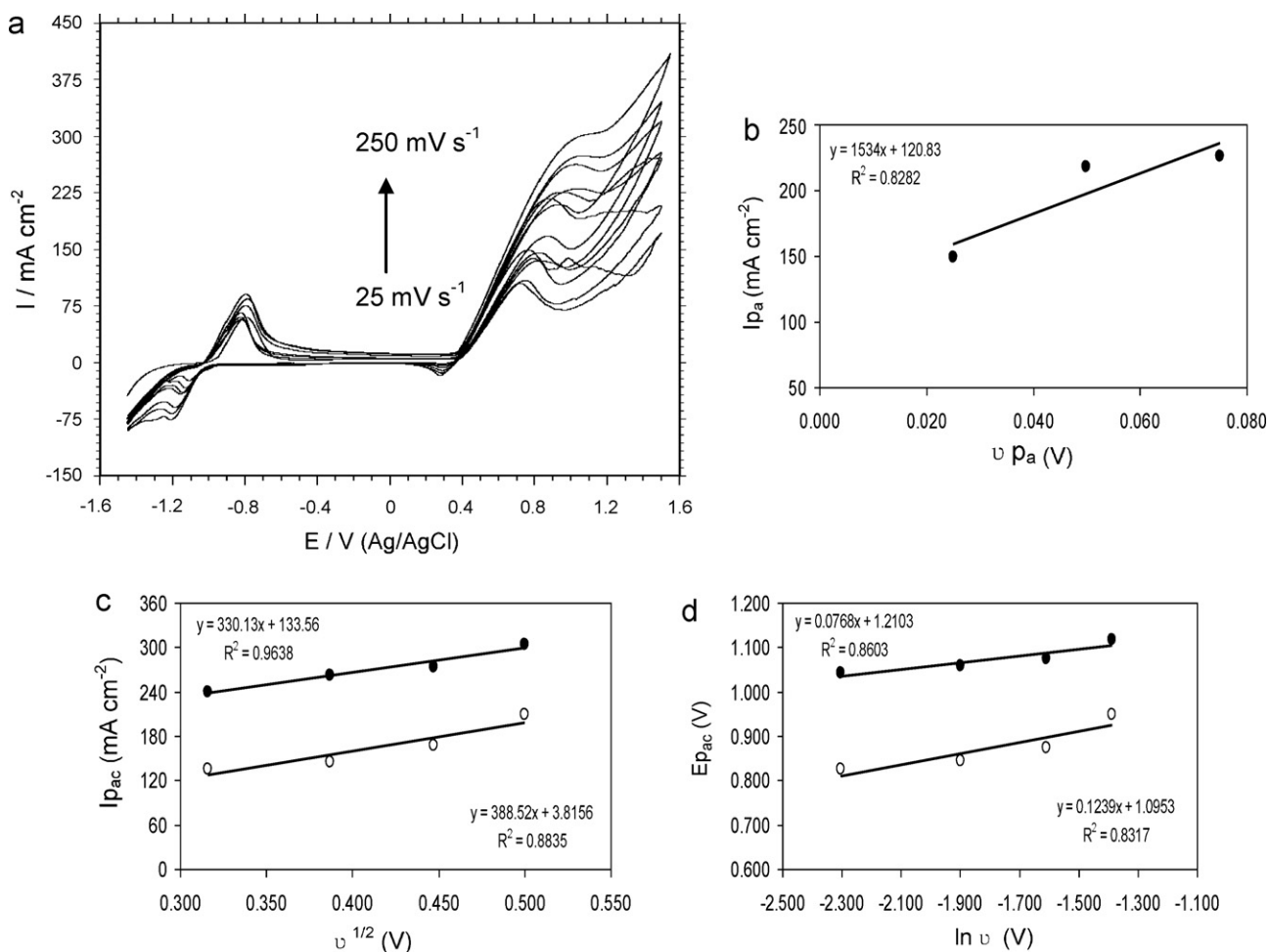
Fig. 7. Effect of the different scan rates (250, 200, 150, 100, 75, 50 and 25 \text{mV s}^{-1} ) on the electrooxidation of 1.00 M \text{CH}_3\text{OH} in 1.00 M KOH at the Ni-promoted Cd/C at 25 °C (a). Dependence of anodic peak current during the forward scan on anodic peak potentials (b). Dependence of anodic (●) and cathodic (○) peak current during the forward and reverse scan on the square roots of scan rate (c). Dependence of both anodic (●) and cathodic (○) E_p on \ln v (d).
